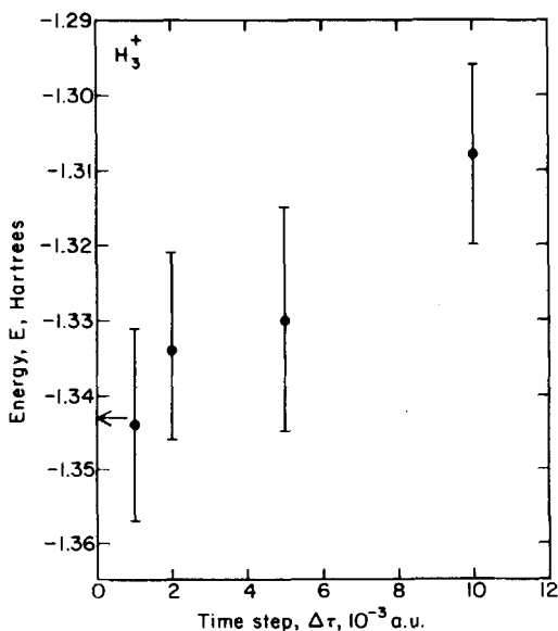
FIG. 2. Variation of total energy with time-step size. The arrow indicates the energy of the lowest variational calculation (Salmon and Poshusta, Ref. 19).
